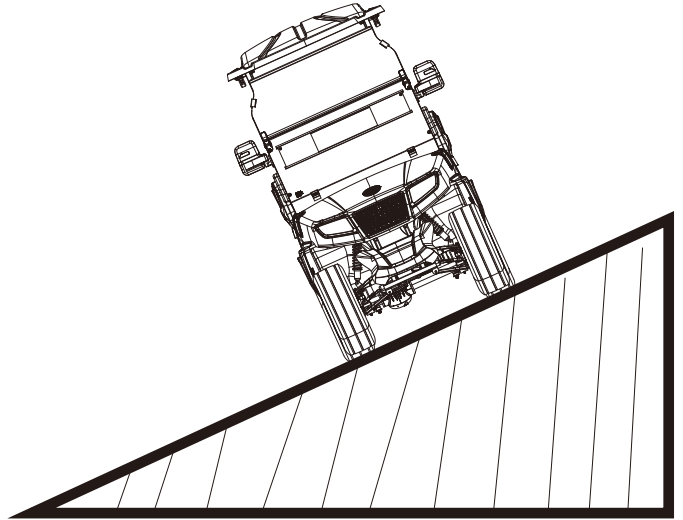
Recommended Max Side Tilt 25% Grade
